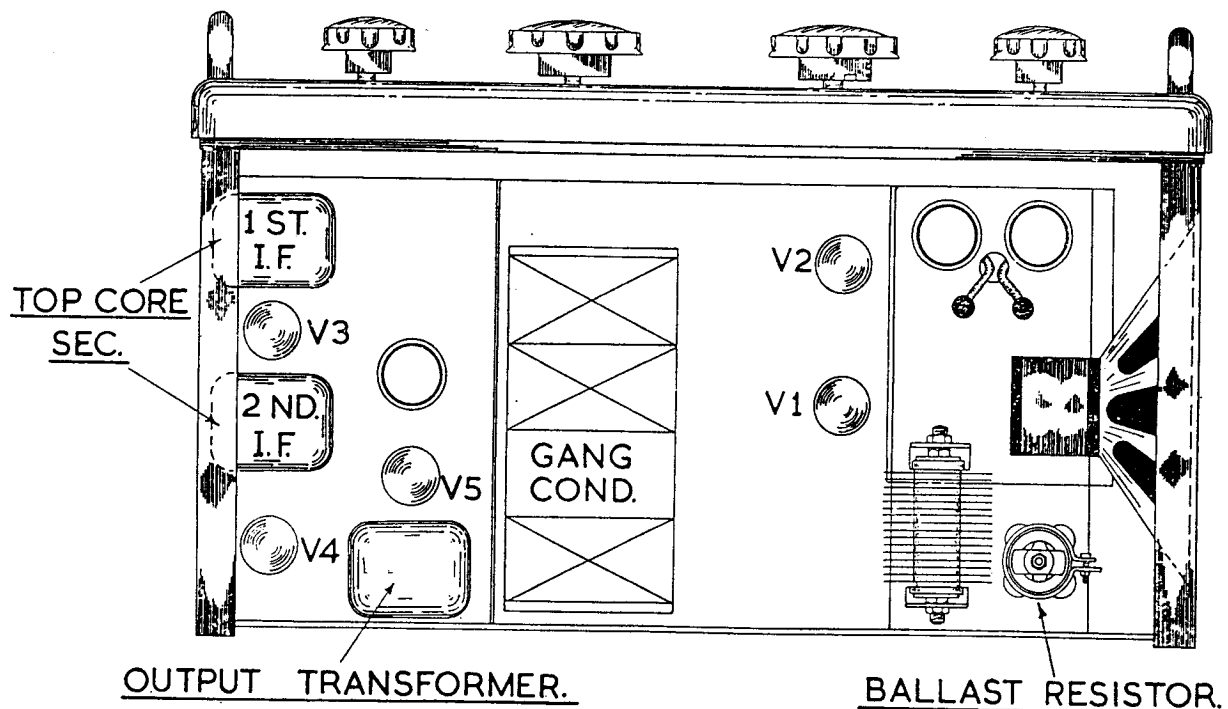
PLAN VIEW OF "670A" RECEIVER IN OUTLINE
